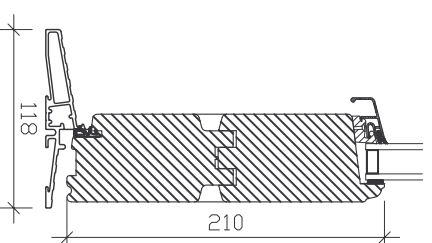
THRESHOLD: LOW LEVEL ALU. INWARD OPENING SASH
