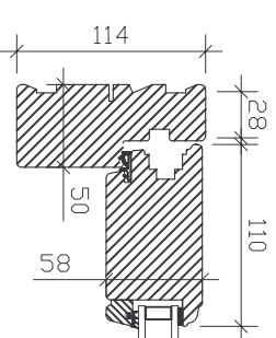
JAMB: OPENING SASH
