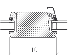
TRANSOM: FIXED SASH
