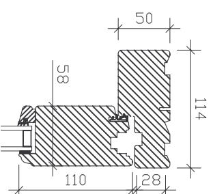
HEAD: OPENING SASH
