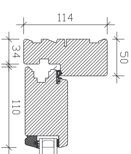
JAMB: OPENING SASH
