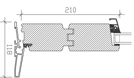
THRESHOLD: LOW LEVEL ALU. OPENING SASH
